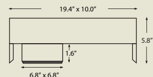
Concrete casting surround
